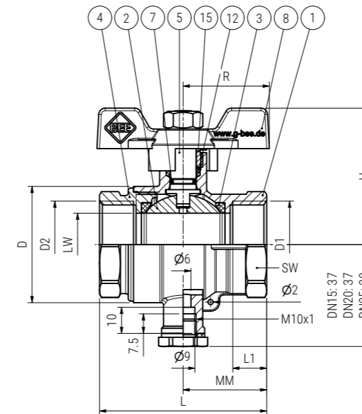
Maßskizze measured sketch
